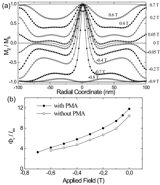
FIG. 3: (a) The evolution of the out-of-plane magnetization as a function of the out-of-plane applied field for a 15 nm thick circular dot of 200 nm in diameter with PMA. (b) The field dependence of the vortex core diameter \phi_V for dots with and without PMA.
