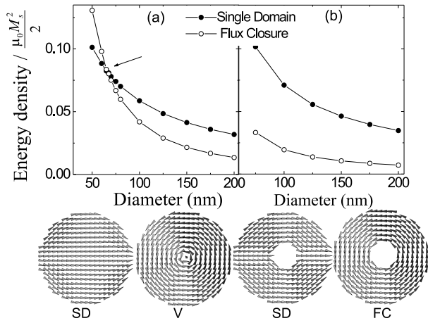
FIG. 1: The variation of the total free energy density as a function of the lateral size of a polycrystalline ( K_u = 0 \text{ J/m}^3 ) 5 nm thick dot (a) and ring (b). The magnetization configuration of the single domain state (SD), the vortex state (V) and the flux closure state (FC).
