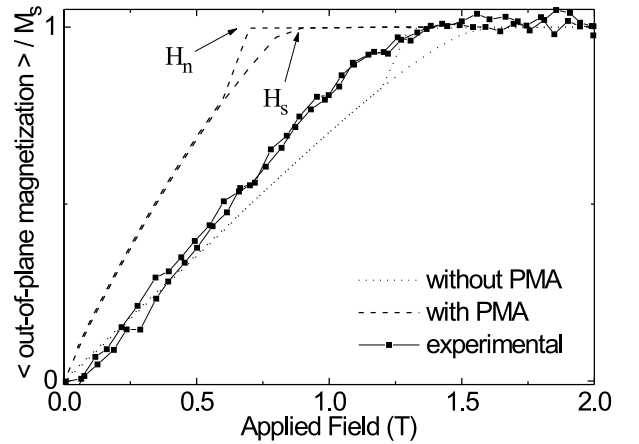
FIG. 2: The simulated perpendicular hysteresis curves of a 15 nm thick circular dot of 200 nm in diameter with PMA, without PMA and as measured experimentally [4].
