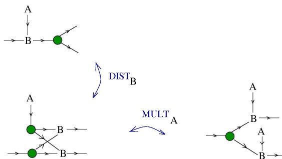
Figure 9: Propagator made from a multiplier and a distributor of the first kind
