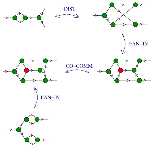
Figure 15: the bit is a propagator
