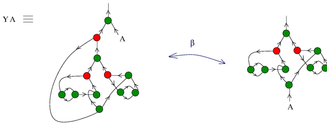
Figure 12: the YA combinator molecule and a first beta move
