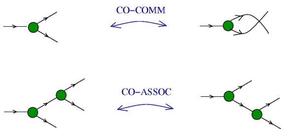
Figure 4: the co-associativity and co-commutativity moves
