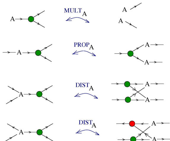
Figure 8: Definition of self-multipliers, propagators, distributors
